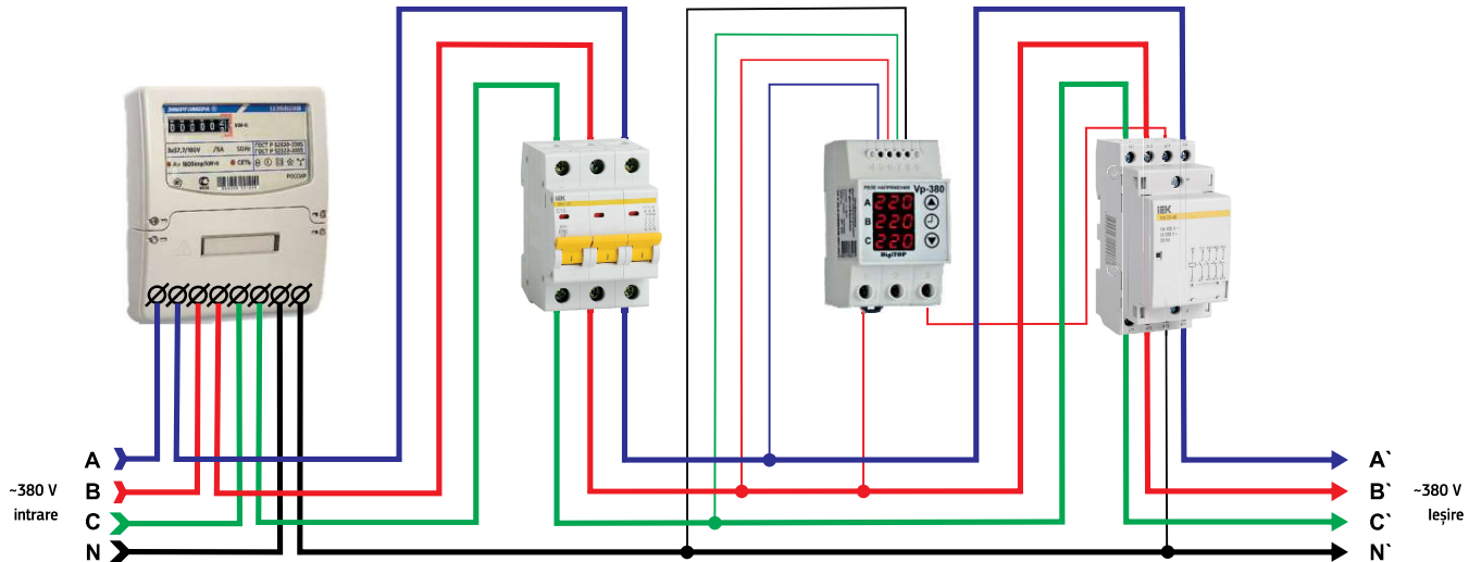
3 protectii-consumatori trifazati
