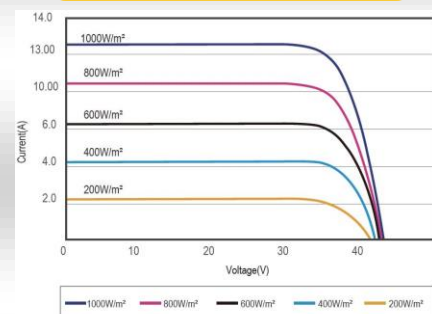
I-V Curves(540W)
