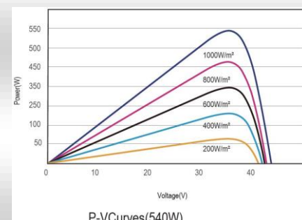
P-V Curves(540W)
