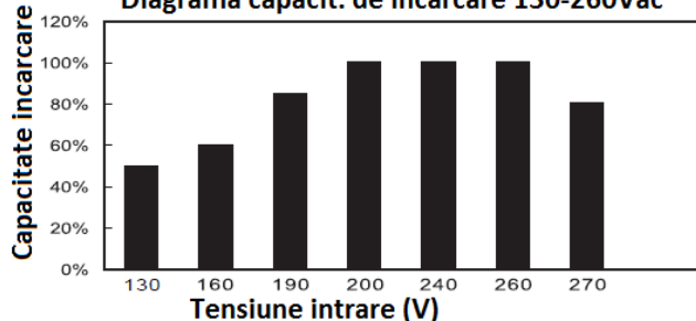
Diagrama capac. de incarcare 130-260Vac
