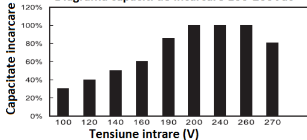
Diagrama capac. de incarcare 100-260Vac
