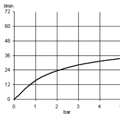
Flow rate diagram
