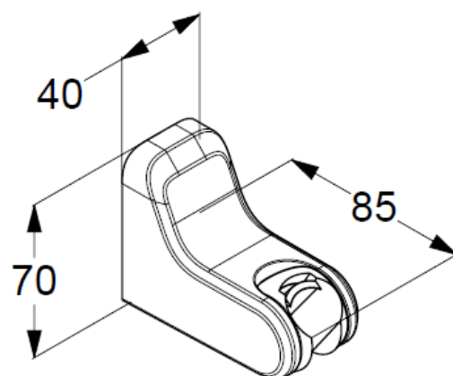
Dimensional drawing
