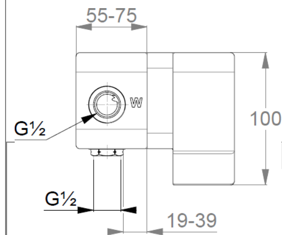
Dimensional drawing
