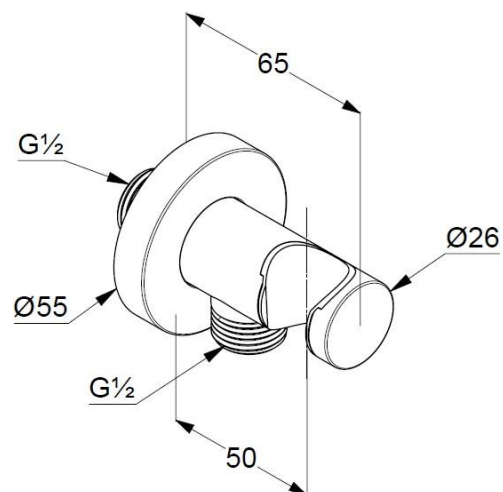
Dimensional drawing
