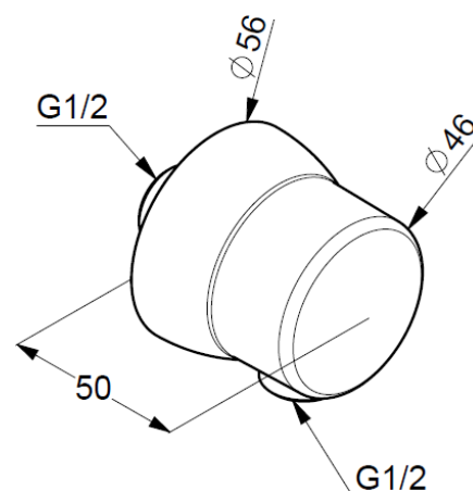
Dimensional drawing
