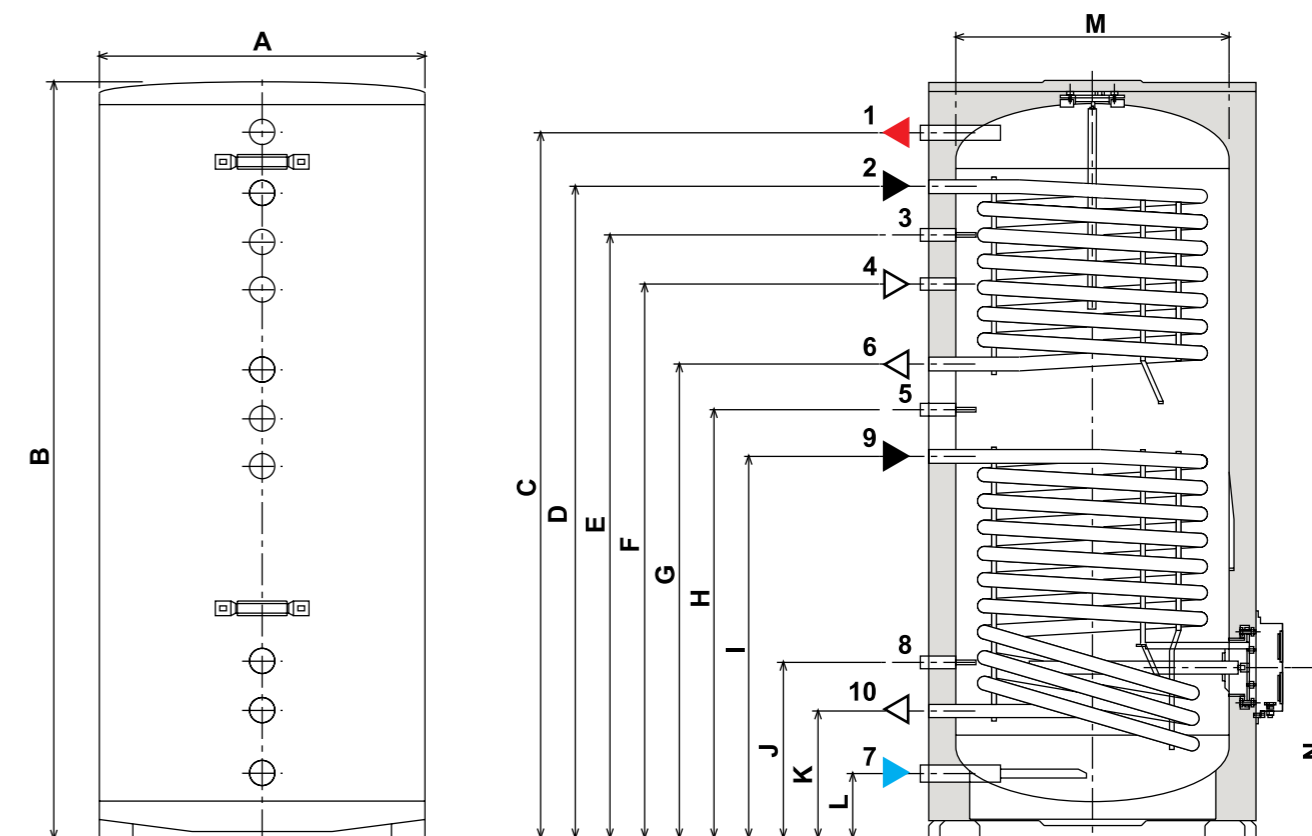
fig.4 - ECOUNIT F 1C
